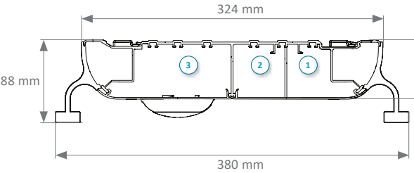
Fluidys Duo (Rails)
