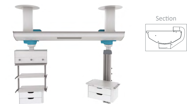
HI-CARE suspended beam configuration with horizontal and vertical box
