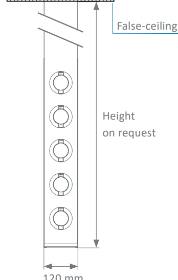
Medical gas casing without fitting
